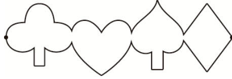
Figure 3: Target shape and its decomposition into upper and lower components.
