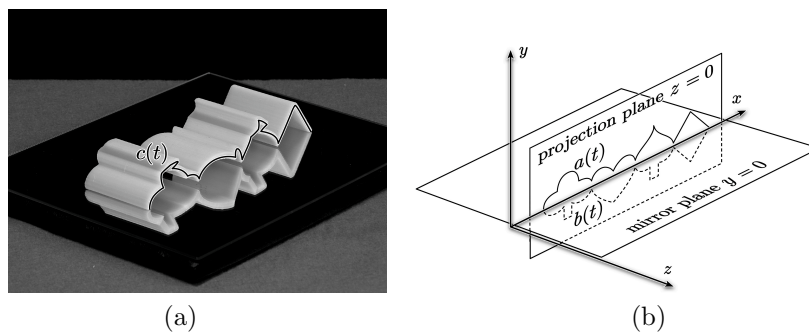
Figure 2: Situation seen from a general viewpoint: (a) another view of the object in Fig. 1; (b) spatial configuration of the input.
